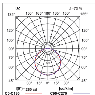
ARTSHAPE SQ LED SMALL FULL ZAW 4500LM PLX 840 Z-1,5M
